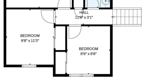
2nd floor
